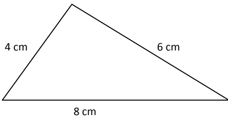
Scalene triangle
