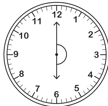
Straight angle
