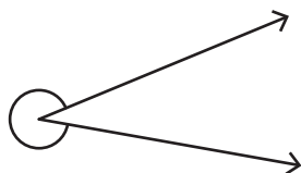
Reflex angle
