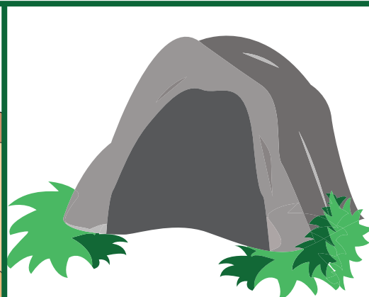
cave
