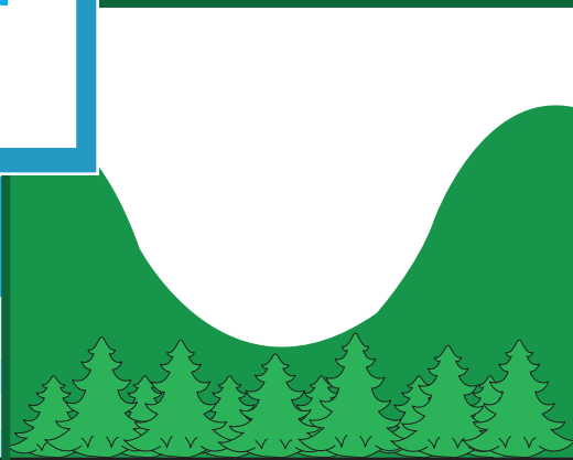
valley
