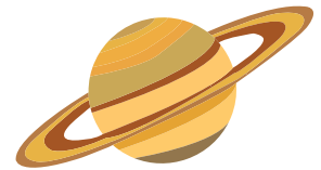
Saturn
