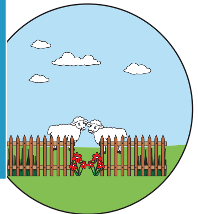
greenery
