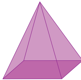
Rectangular Pyramid
