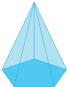
Pentagonal Pyramid
