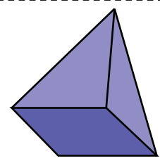
Square pyramid
