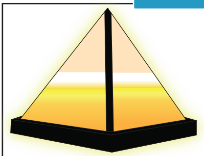
square pyramid
