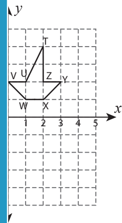
Reflection across the line x = -1
