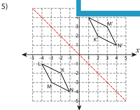
Reflection across the line y = -x
